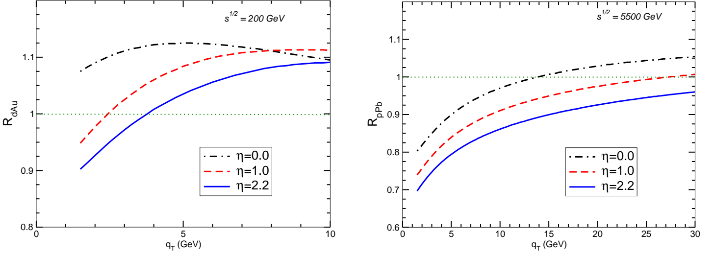
Fig. 3. Nuclear modification ratio for D mesons in d+Au ( \sqrt{s} = 200 GeV) and p+Pb ( \sqrt{s} = 5.5 TeV) processes.
