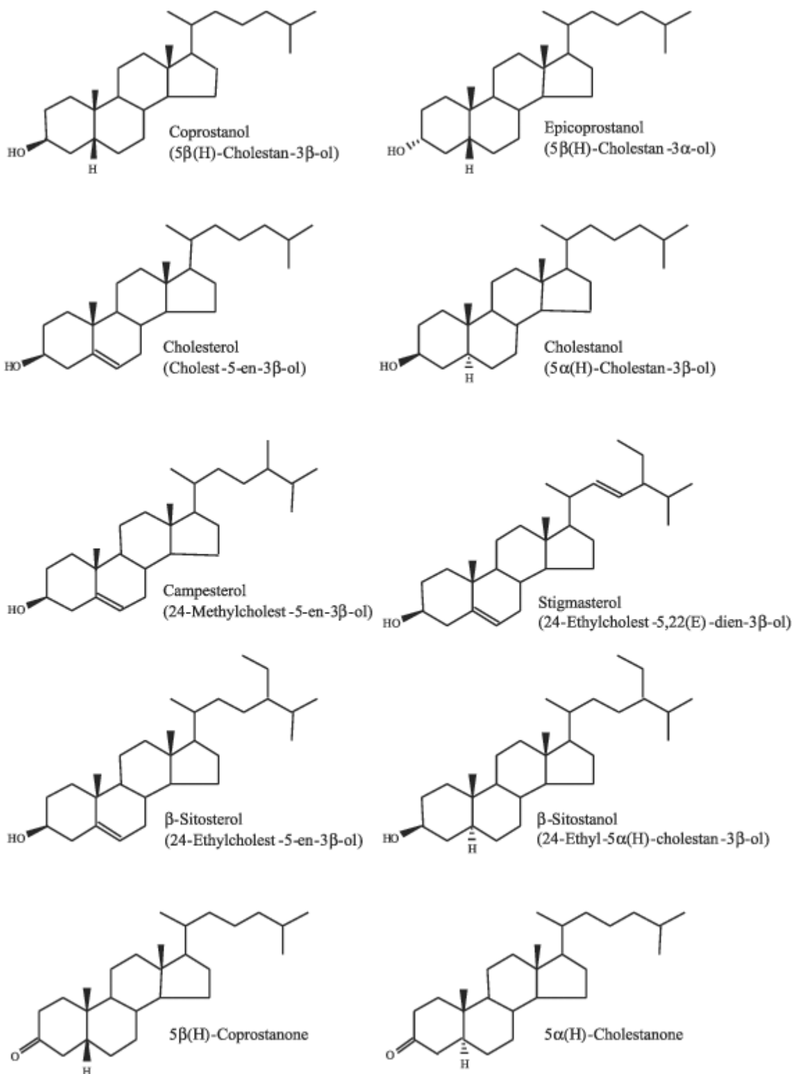
Scheme 1. Chemical structures of sterols and ketones analysed.
