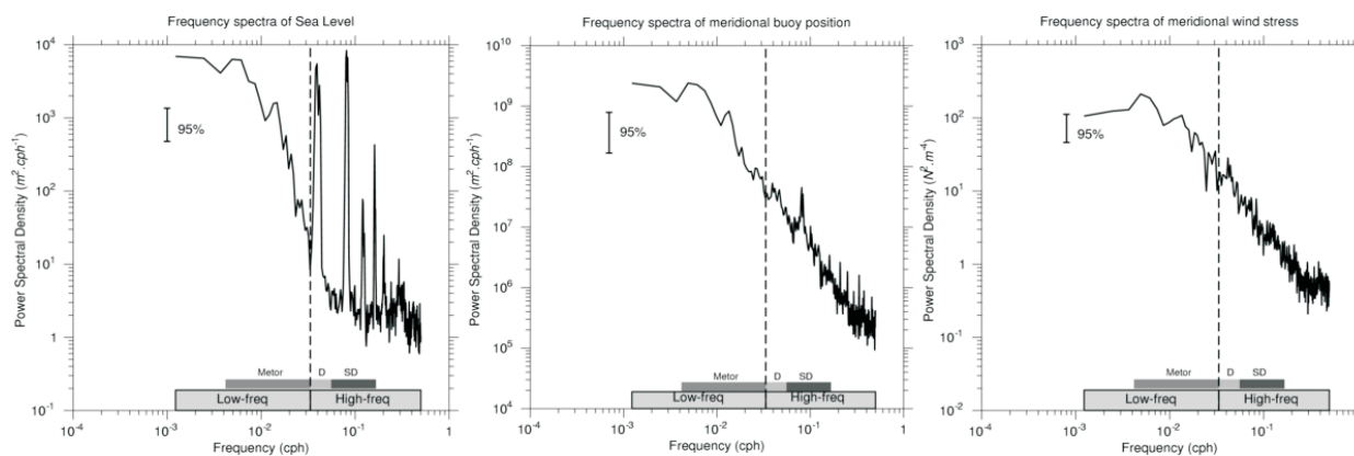
Figure 6. Spectra of sea level (left), buoy meridional displacement (middle) and meridional wind stress (right panel). Low and high-frequency bands as well as Meteorological forcing (Meteor), diurnal(D) and semi diurnal (SD) sub-bands are indicated.
