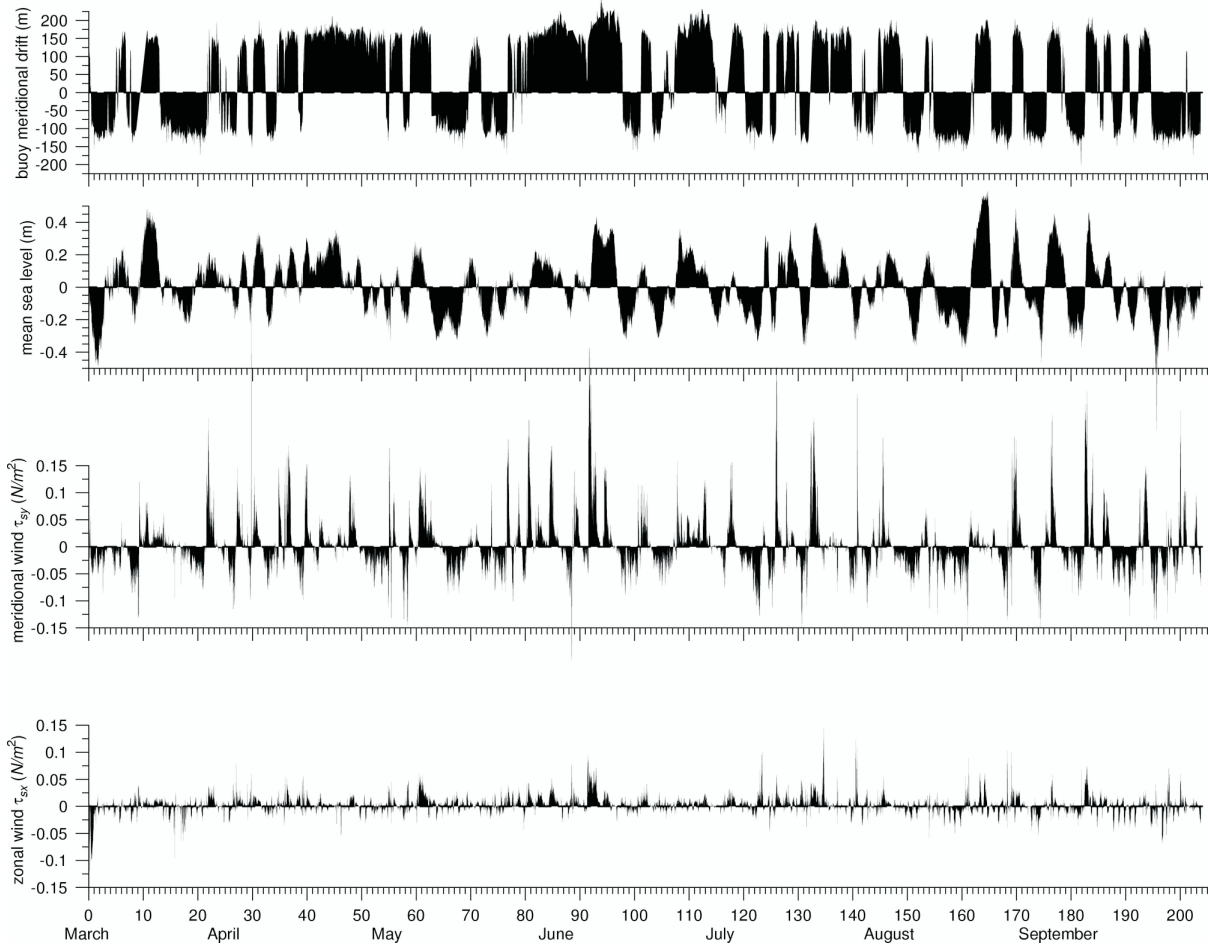
Figure 4. Time series of meridional waverider position, mean sea level, meridional wind stress and zonal wind stress for the period between March 21 th and October 11 th 2002. Time is depicted in days.
