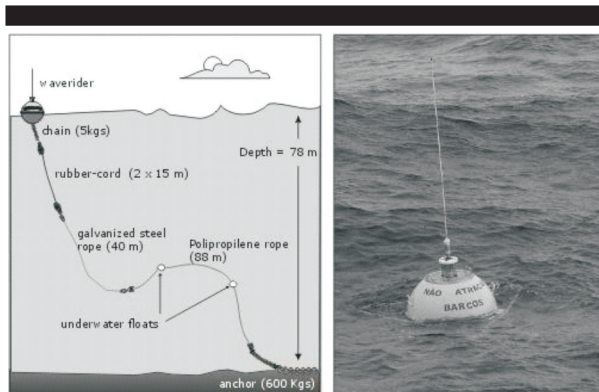
Figure 2. Waverider mooring line scheme (left) and waverider in operation (right). The mooring length adds to almost twice the local depth.
