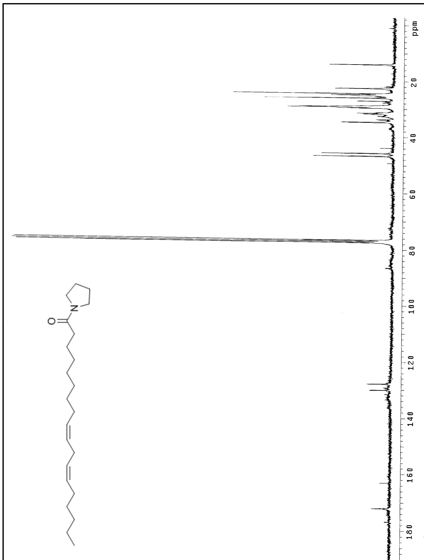
Espectro 53 – RMN ^{13}\text{C} (75 Hz, \text{CDCl}_3 ) da N -pirrolidil-9,12- Z -octadidecenamida (71e).
