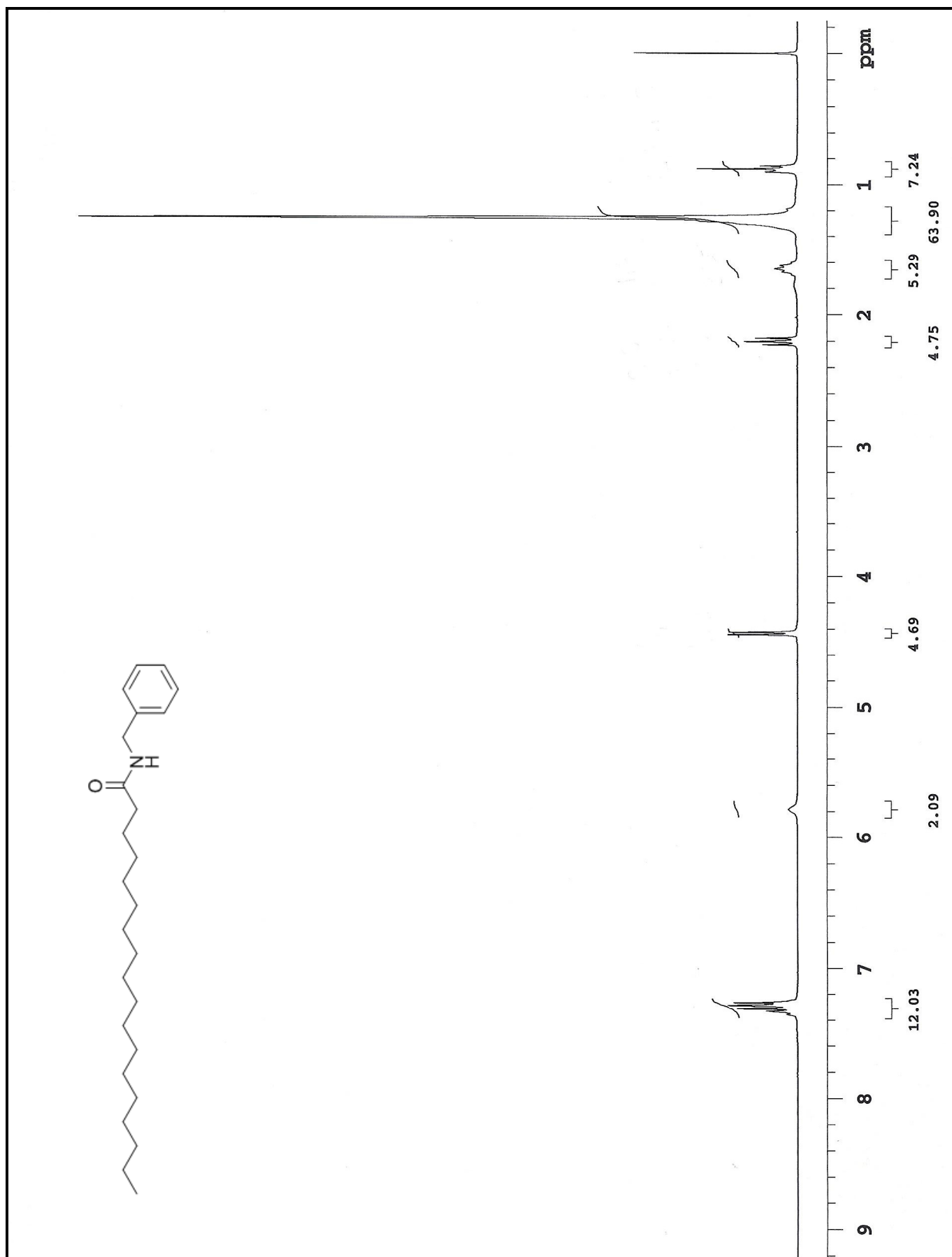
Espectro 11 – RMN ^1\text{H} (300 Hz, \text{CDCl}_3 ) da N -benzil-octadecanamida (66b).
