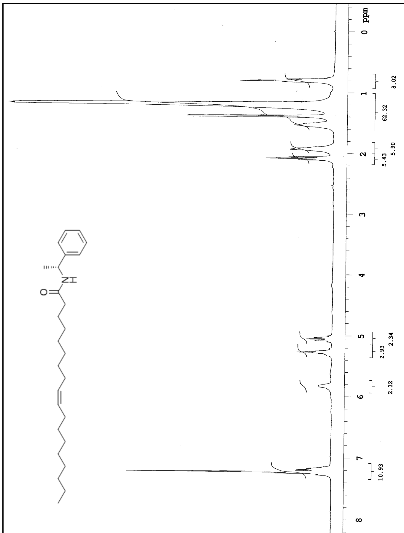
Espectro 38 – RMN ^1\text{H} (300 Hz, \text{CDCl}_3 ) da \alpha -metil-N-benzil-9-Z-octadecenamida (67c).
