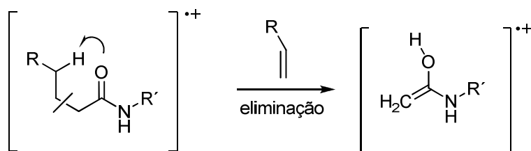
Figura 28 - Rearranjo de McLafferty.
