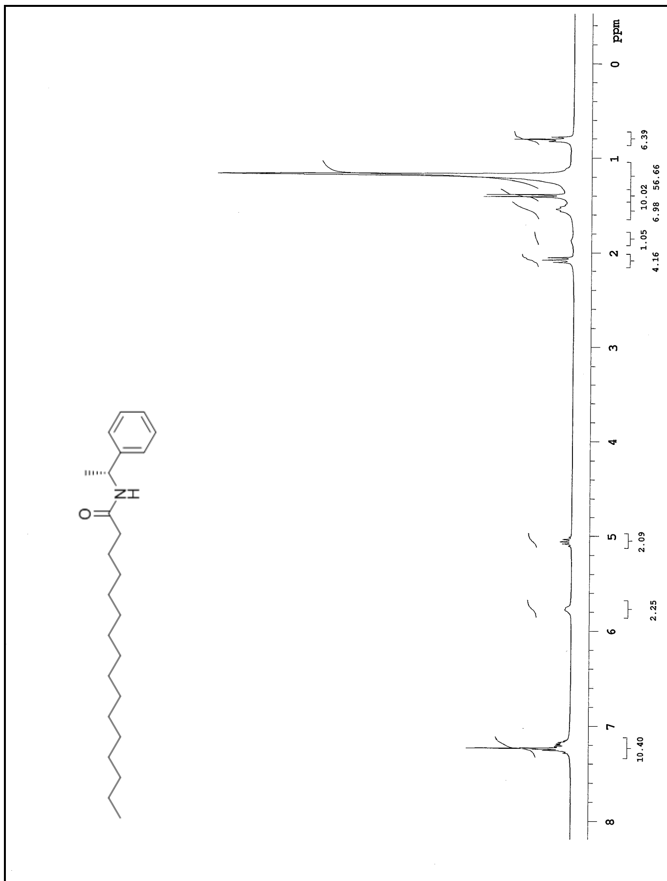
Espectro 30 – RMN ^1\text{H} (300 Hz, \text{CDCl}_3 ) da \alpha -metil-N-benzil-hexadecanamida (67a).
