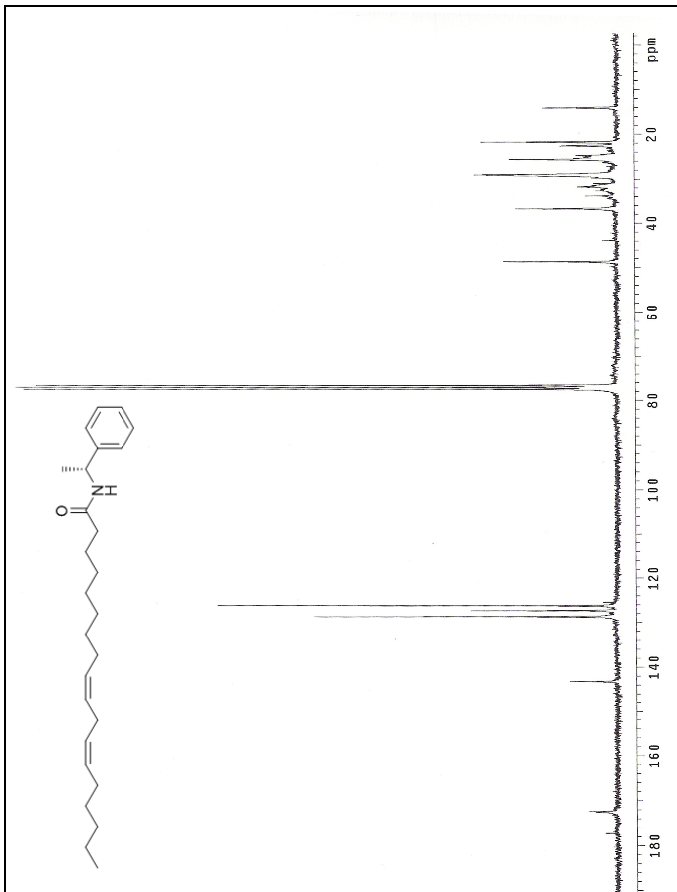
Espectro 49 – RMN ^{13}\text{C} (75Hz, \text{CDCl}_3 ) da \alpha -metil- N -benzil-912- Z -octadidecenamida (67e).
