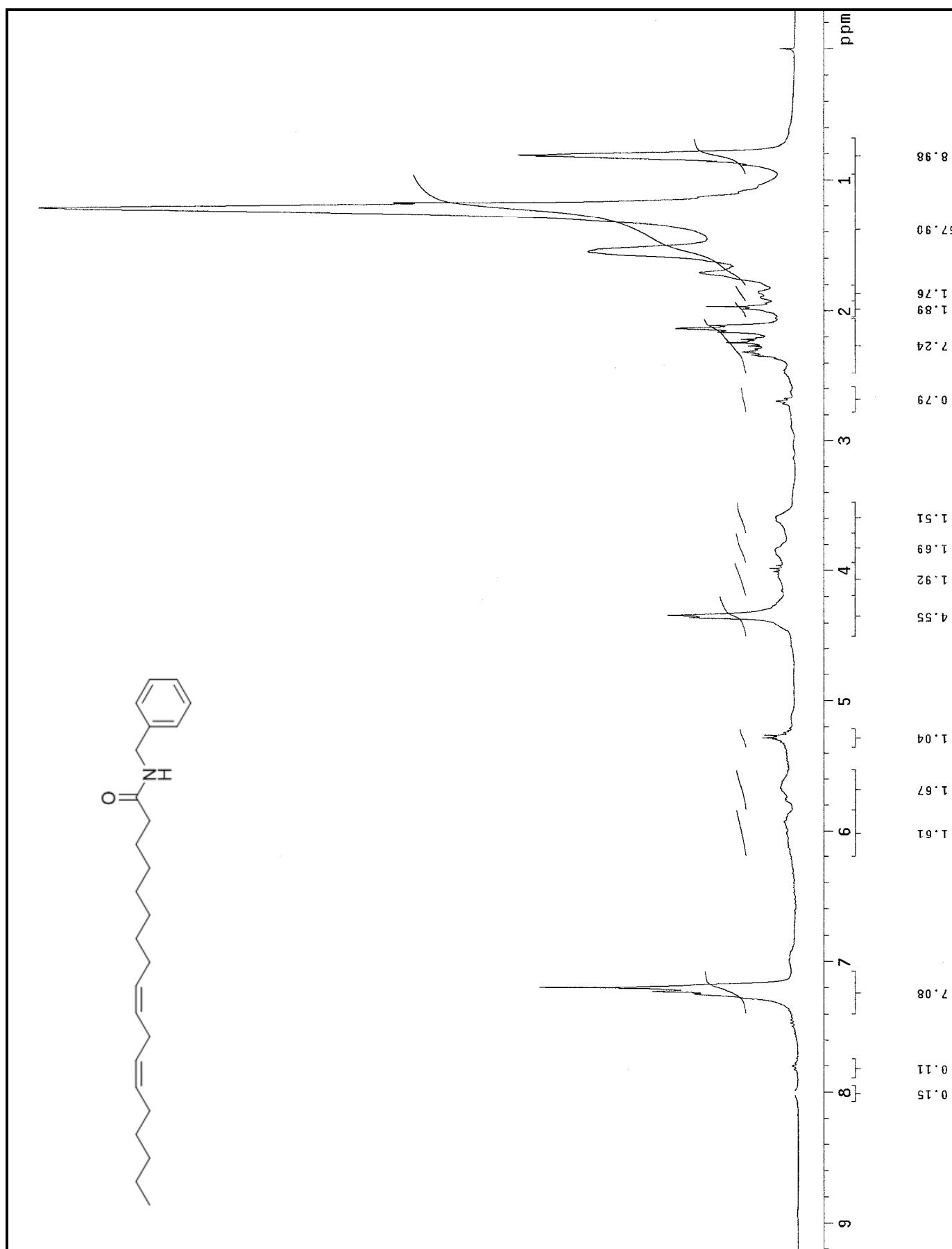
Espectro 25 – RMN ^1\text{H} (300 Hz, \text{CDCl}_3 ) da N -benzil-9,12- Z -octadidecenamida (66e).
