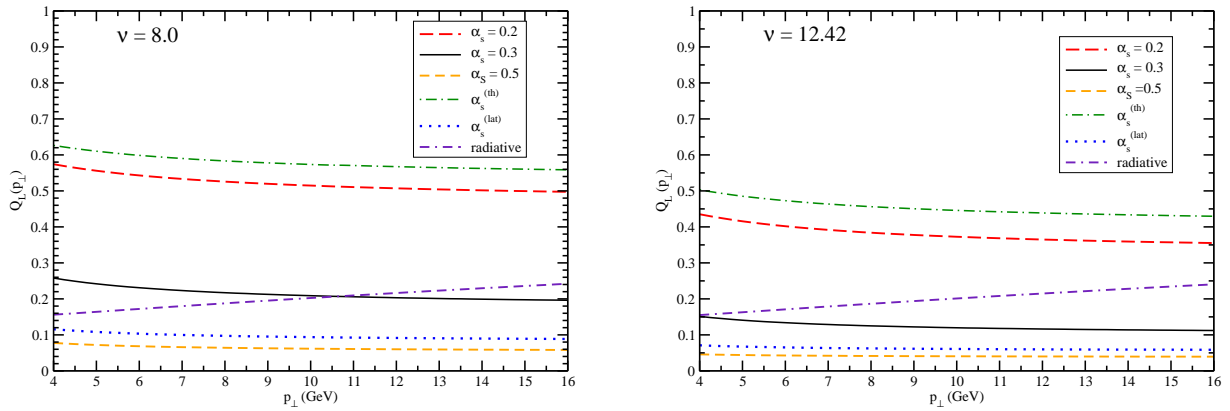
Fig. 6. Quenching factor for light quark p_{\perp} -spectrum. An estimative of radiative energy loss is presented for comparison. The left panel presents results with \nu = 8.0 in the vacuum spectrum parametrization, while results with \nu = 12.42 are presented in the right panel.
