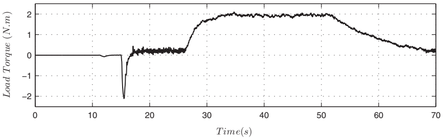
Fig. 6. FLC control with 36 rad/s rotor speed reference
